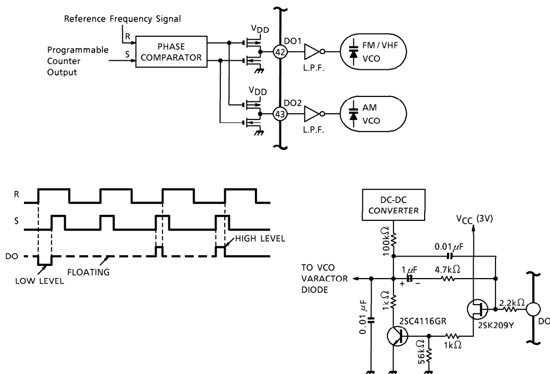
DO Output Timing Chart
