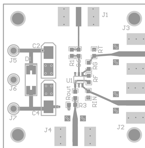
Figure 49. Layer1 Silk (SOT-23 Board Layout)
