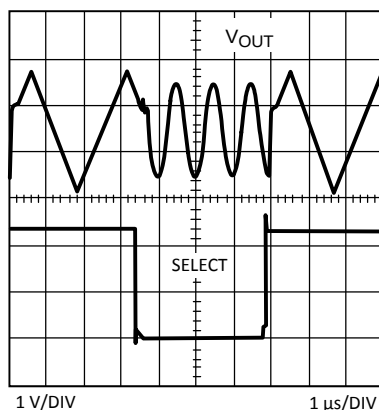
Figure 47. 2:1 MUX Output
