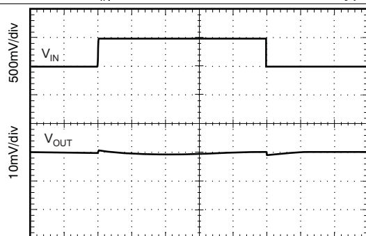
Time (400µs/div) C_{LOAD} = 10\text{ }\mu\text{F} , I_{OUT} = 0\text{ mA}
