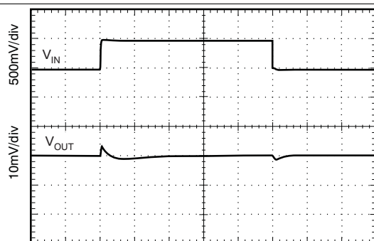
Time (200µs/div) C_{LOAD} = 10\text{ }\mu\text{F} , I_{OUT} = 1\text{ mA}
