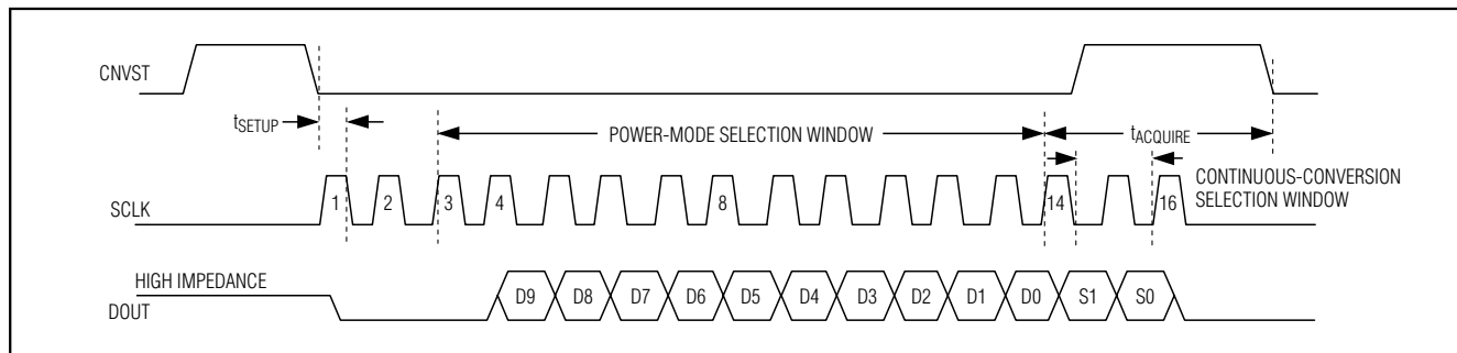
Figure 5. Interface-Timing Sequence
