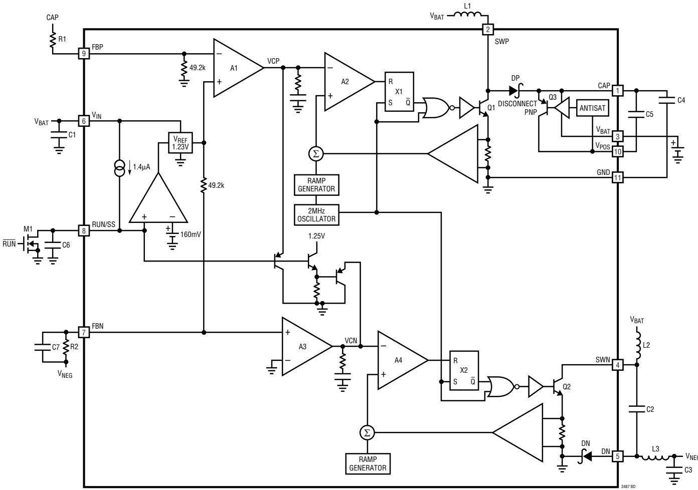
Figure 1. Block Diagram
