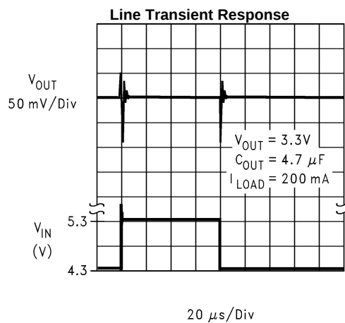
20 \mu\text{s}/\text{Div} Figure 16.
