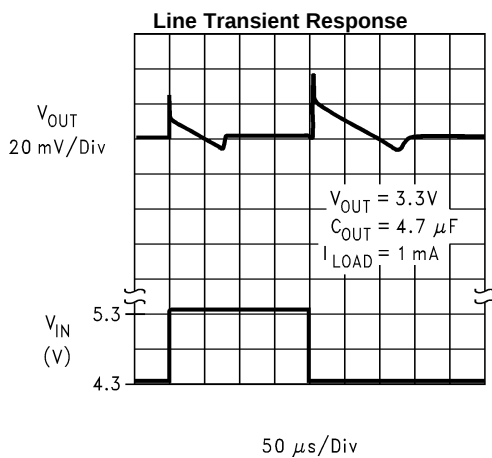
50 \mu\text{s}/\text{Div} Figure 15.
