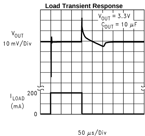
50 \mu\text{s}/\text{Div} Figure 14.
