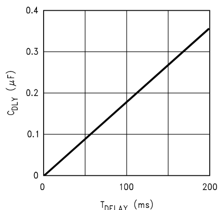
Figure 47. Plot of C_{\text{DLY}} vs T_{\text{DELAY}}
