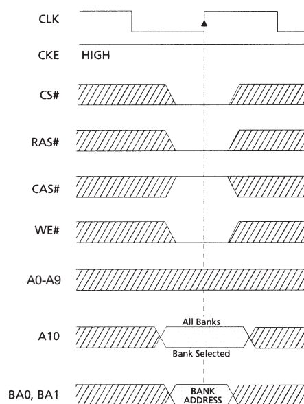
FIGURE 20: PRECHARGE Command
