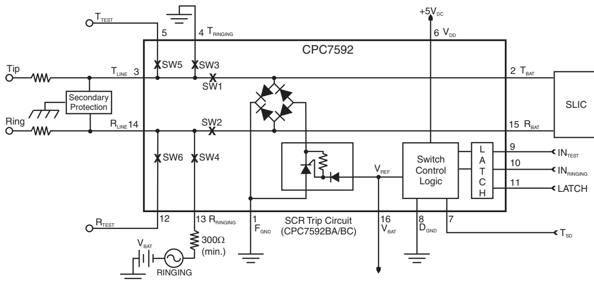
Figure 1. CPC7592 Block Diagram
