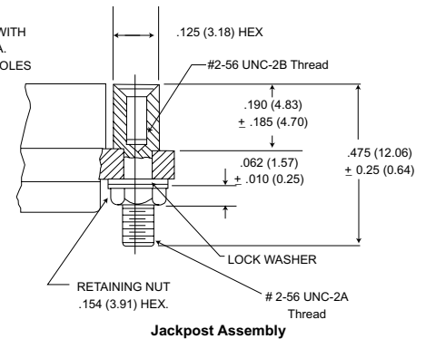
Jackpost Assembly
