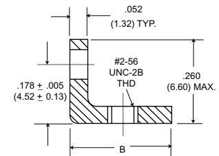
Jackpost - (P)
