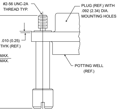
Figure 2. Jackscrew - High Profile Slotted Head Size 9-51 Size 100*
