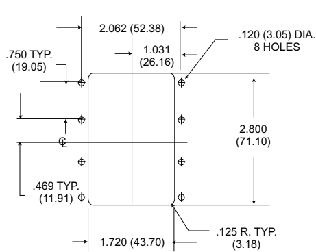
- 33 FRONT MOUNT
