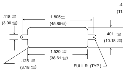
Figure 2 Rear Mounting
