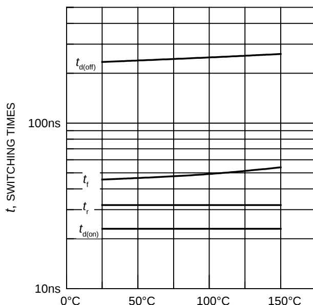
Figure 11. Typical switching times as a function of junction temperature
