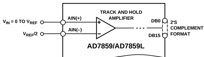
Figure 13. \pm V_{REF}/2 about V_{REF}/2 Bipolar Input Configuration
