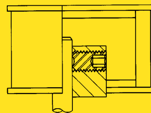
Internal Knurl Point
