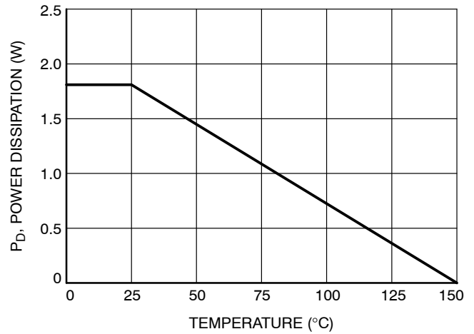
Figure 12. Power Derating
