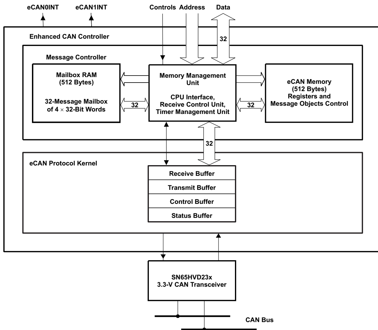
Figure 6-35. eCAN Block Diagram and Interface Circuit
