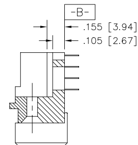
SECTION W-W
