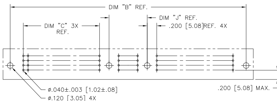
SECTION U-U
