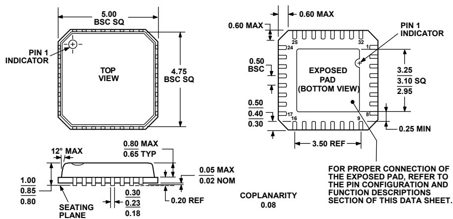
COMPLIANT TO JEDEC STANDARDS MO-220-VHHD-2 Figure 64. 32-Lead Lead Frame Chip Scale Package [LFCSP_VQ] 5 mm x 5 mm Body, Very Thin Quad (CP-32-2) Dimensions shown in millimeters
