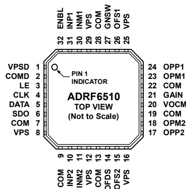
Figure 4. Pin Configuration
