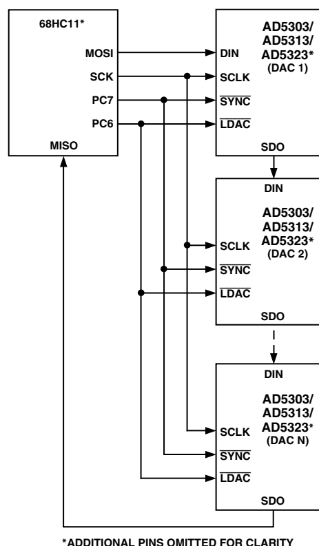
Figure 22. Daisy-Chain Mode
