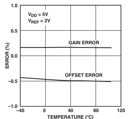
TPC 9. Offset Error and Gain Error vs. Temperature
