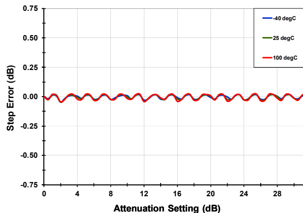
DNL [1900 MHz]
