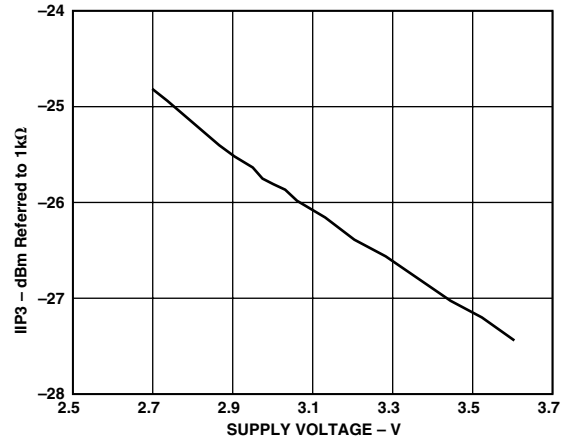
Figure 15. IF Amplifier Input IP3 vs. Supply Voltage
