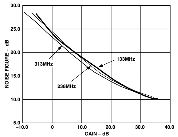
Figure 17. IF Amplifier Noise Figure vs. Gain
