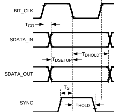
Data Delay, Setup and Hold
