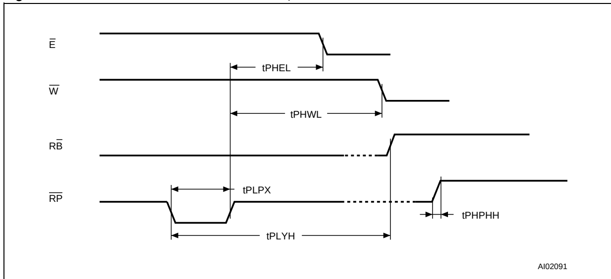
Figure 11. Read and Write AC Characteristics, \overline{RP} Related
