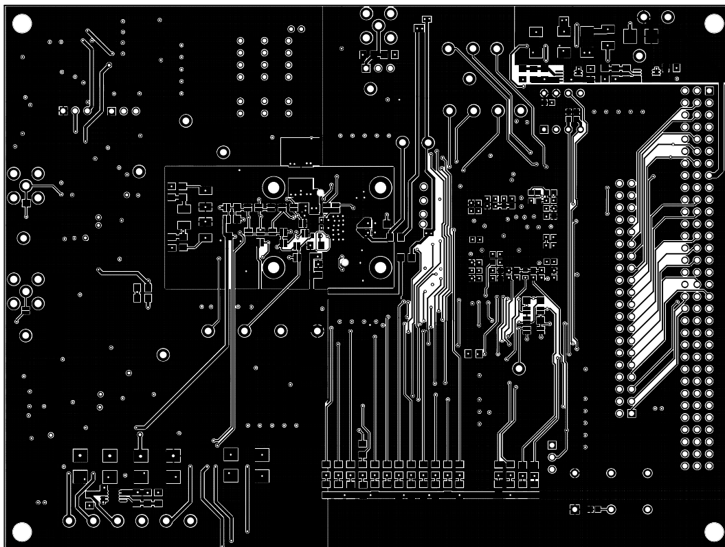
Figure 15. Bottom Side Layer
