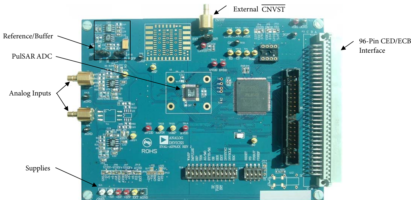
Figure 1. Evaluation Board
