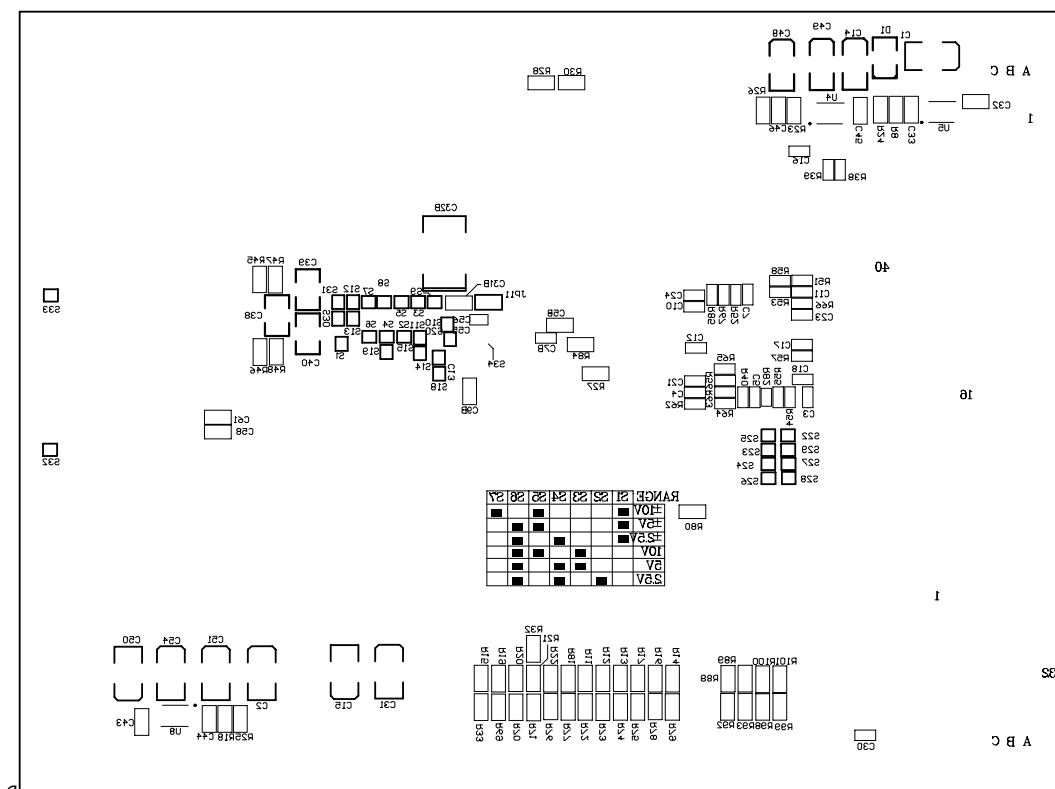
Figure 16. Bottom Side Silk-Screen
