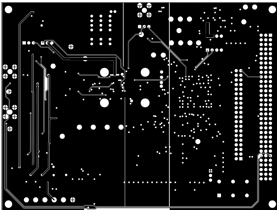
Figure 14. Shield Layer
