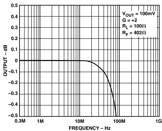
TPC 9. 0.1 dB Flatness
