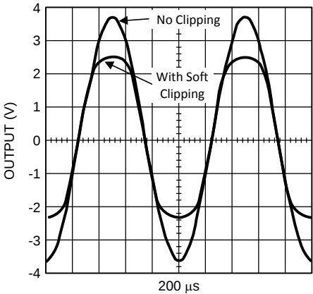
Figure 22. Soft Clipping vs No Clipping
