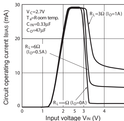
Fig.37 Circuit Operating Current vs. Input Voltage (PQ030EZ01ZxH)
