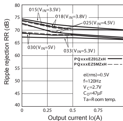
Fig.42 Ripple Rejection vs. Output Current
