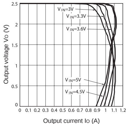
Fig.6 Overcurrent Protection Characteristics (PQ025EZ5MZxH)
