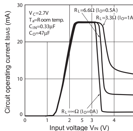
Fig.38 Circuit Operating Current vs. Input Voltage (PQ033EZ01ZxH)
