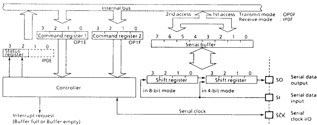
Figure 2-9. Configuration of Serial Interface
