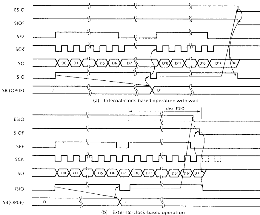
Figure 2-12. 8-bit transmit mode
