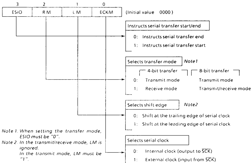
Serial interface control command register 2 (Port address OP1F)
