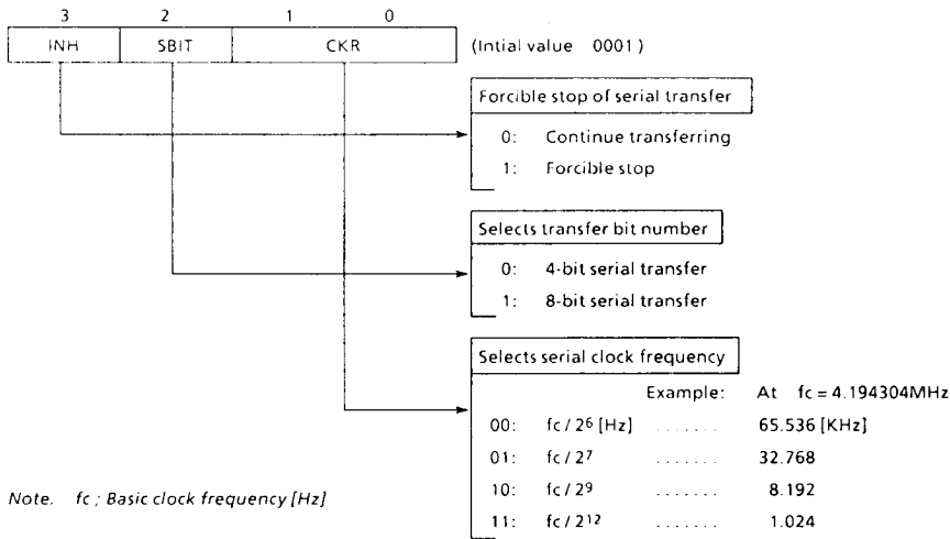
Serial interface control command register 2 (Port address OP1F)
