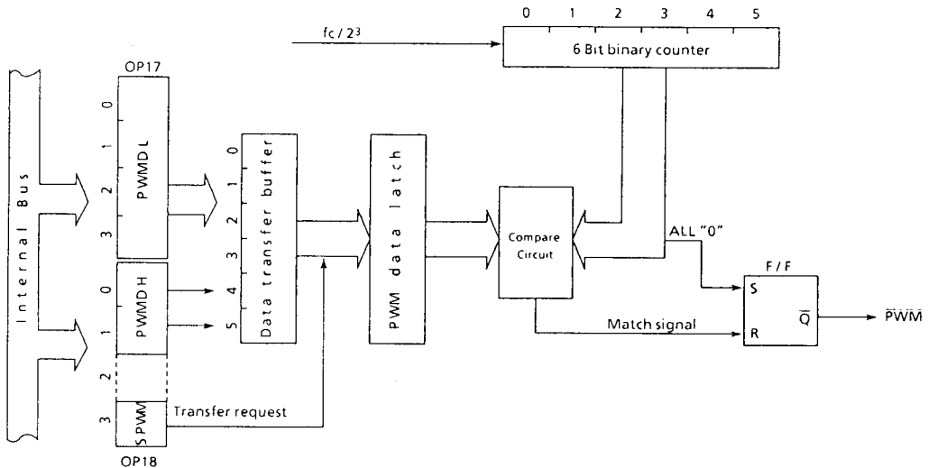
Figure 2-3. PWM output circuit
