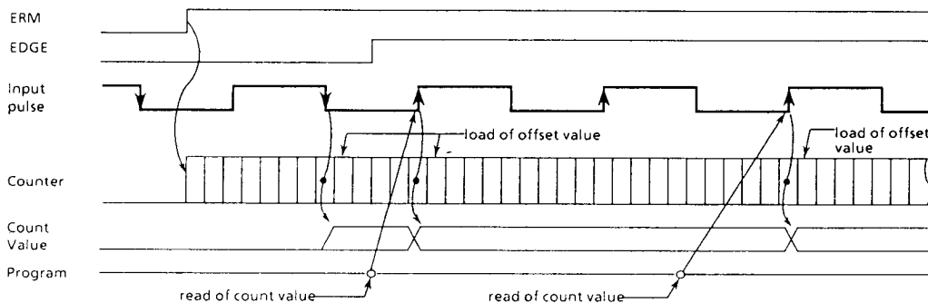
Figure 2-8. Timing chart
