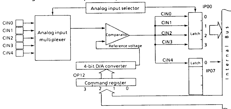
Figure 2-2. Comparator input circuit
