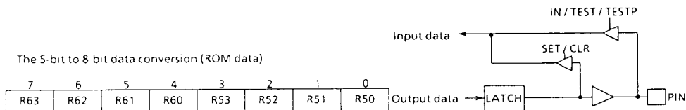
Figure 2-1. Ports R5 and R6
