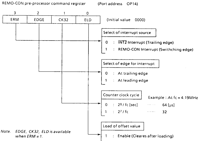
Figure 2-7. Command Register
