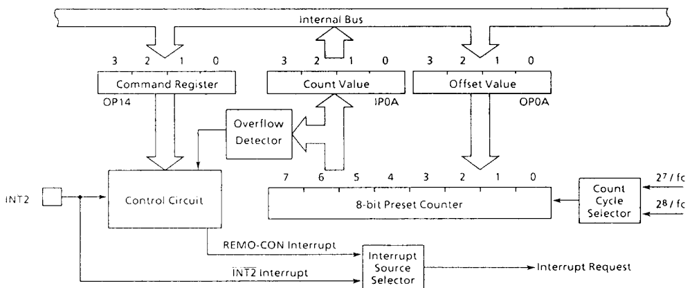
Figure 2-6. Remote Control Pre-processor
