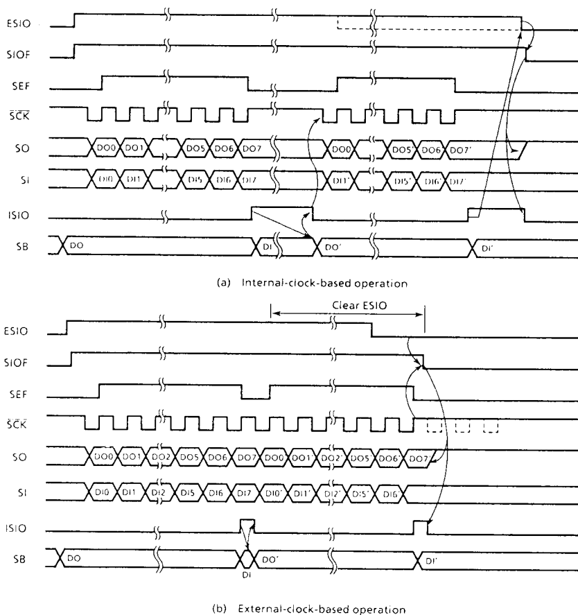
Figure 2-13. 8-bit Transmit / Receive Mode
