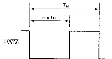
Figure 2-4. \overline{\text{PWM}} output waveform
