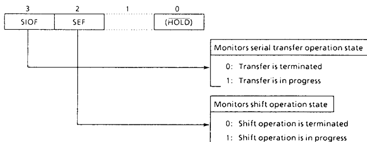
Figure 2-11. Serial Interface Status Register
