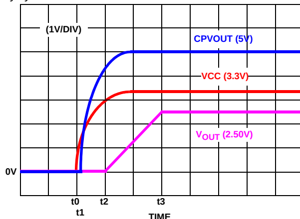
FIGURE 1. SOFT-START INTERVAL
