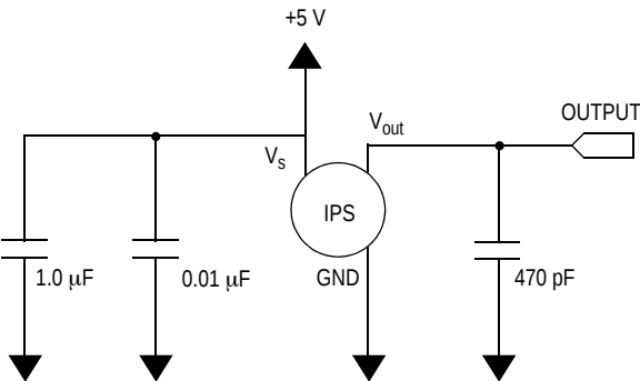
Figure 3. Typical Application Circuit (Output Source Current Operation)
