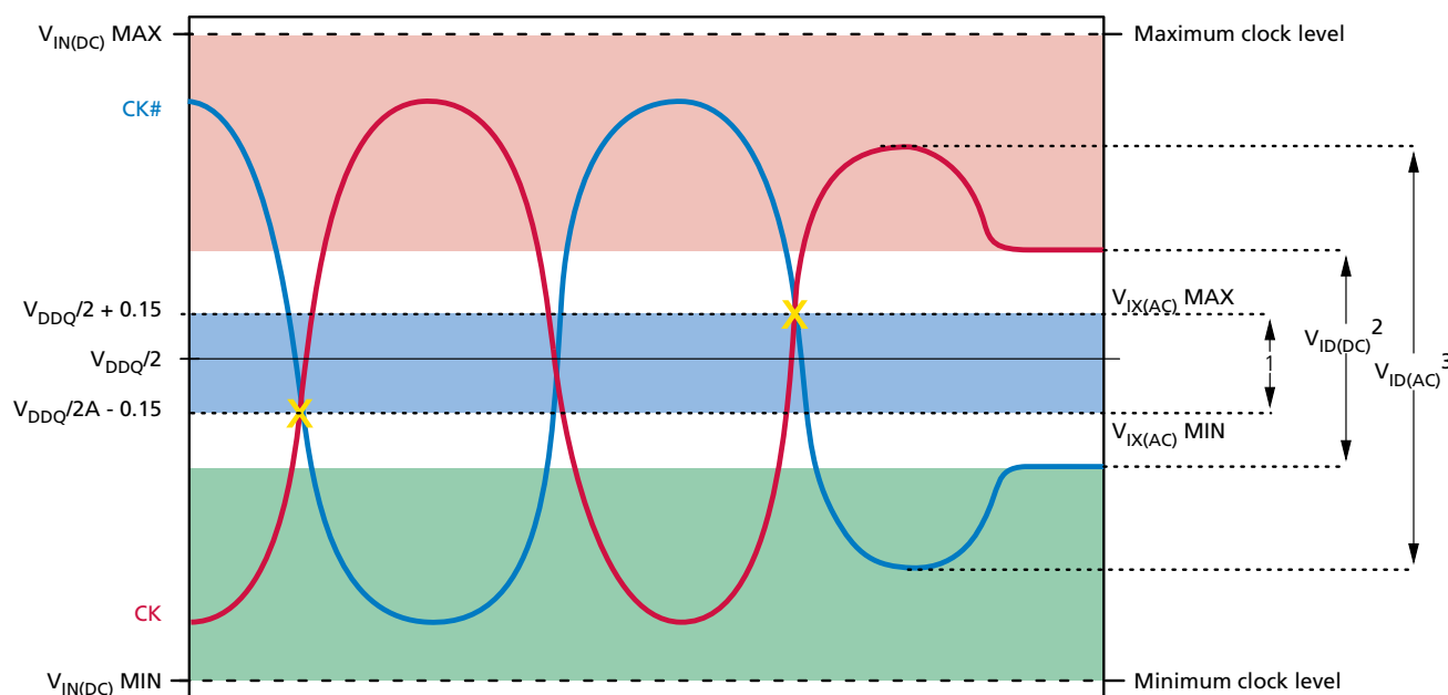
Figure 9: Clock Input
