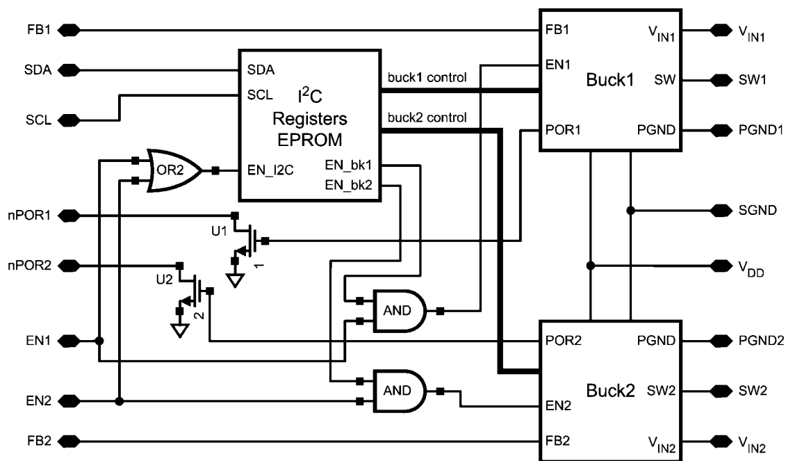
FIGURE 2. Functional Diagram
