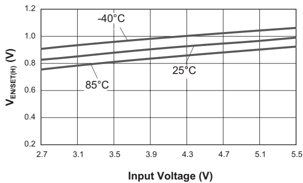
EN/SET, FLEN Input High Threshold vs. Input Voltage
