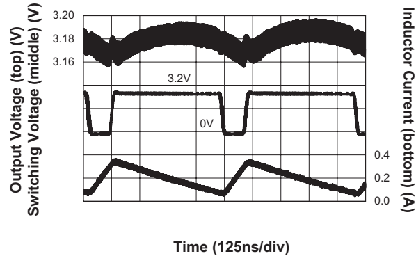
Movie Mode Output Ripple (68.5mA/ch)
