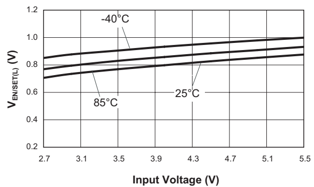
EN/SET, FLEN Input Low Threshold vs. Input Voltage
