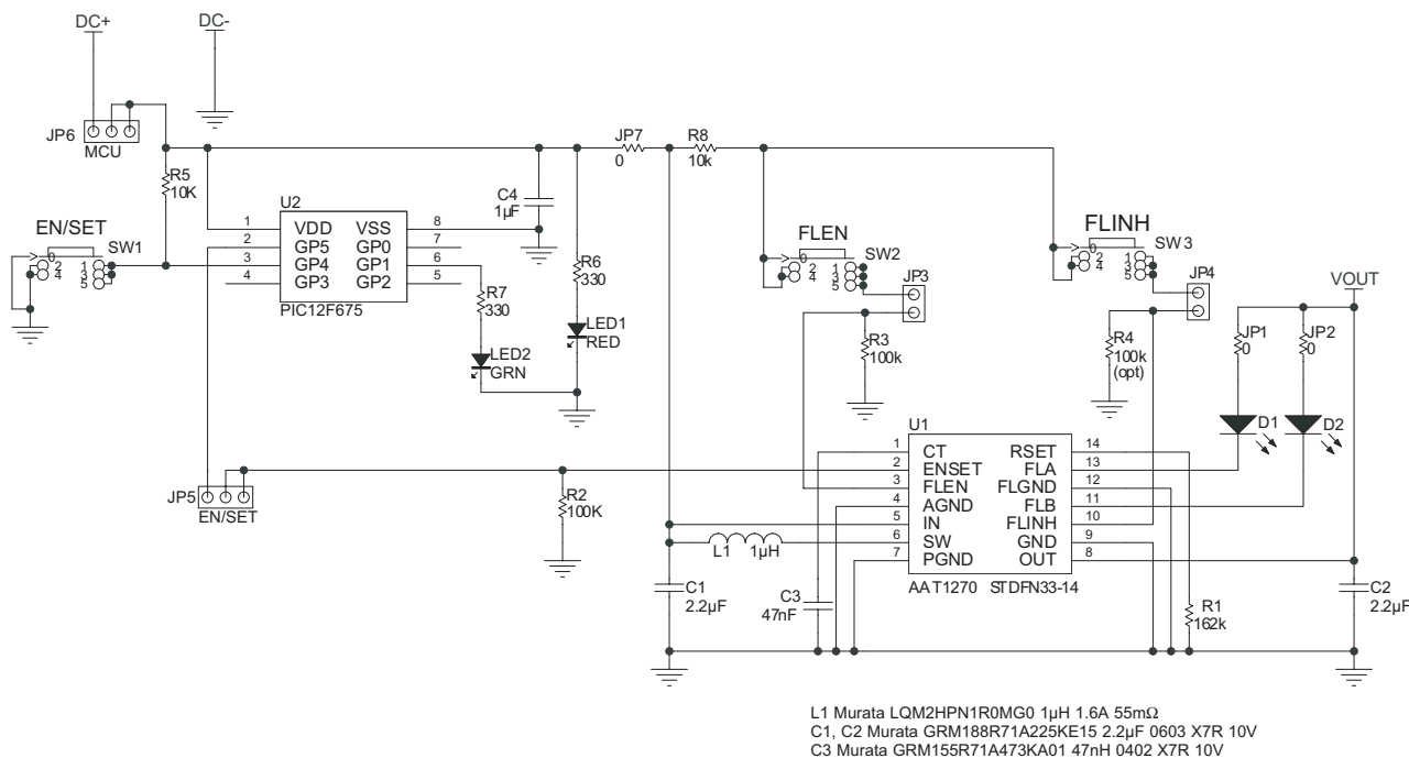
Figure 3: AAT1270 Evaluation Board Schematic.
