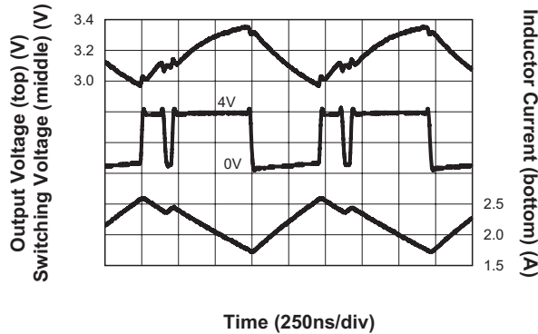
Flash Mode Output Ripple (500mA/ch)
