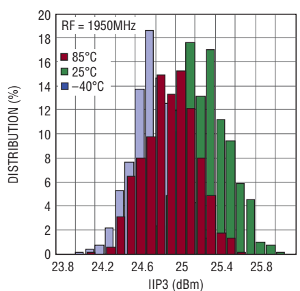
IIP3 Distribution
