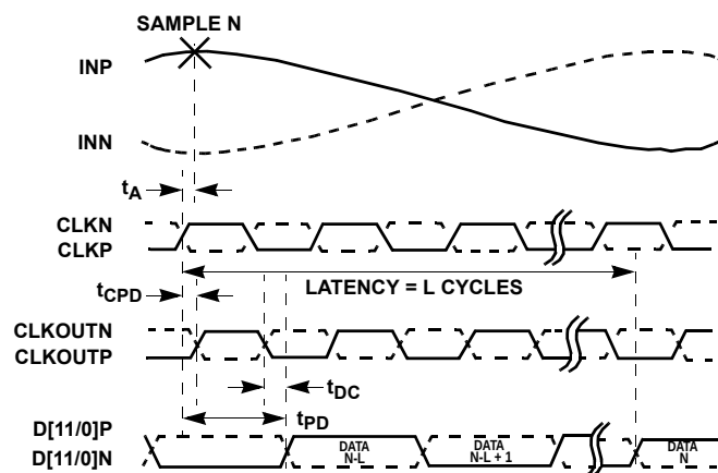
FIGURE 2B. SDR
