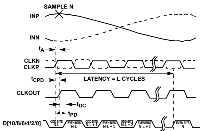
FIGURE 3A. DDR
