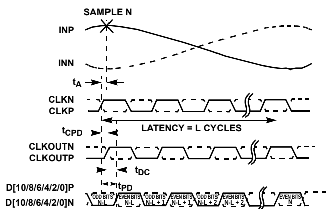
FIGURE 2A. DDR
