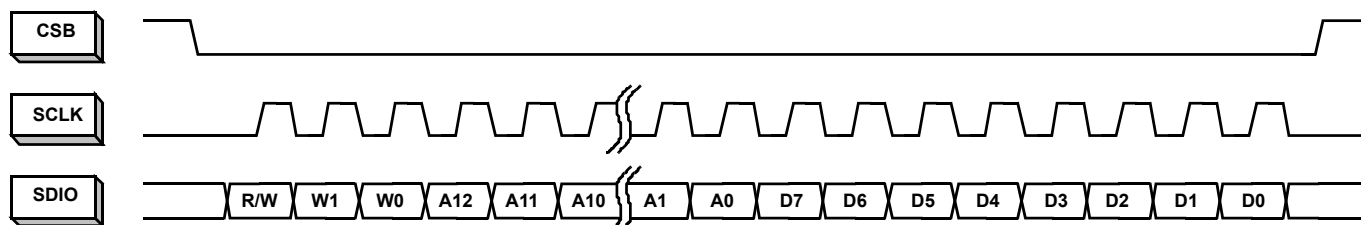
FIGURE 34. MSB-FIRST ADDRESSING
