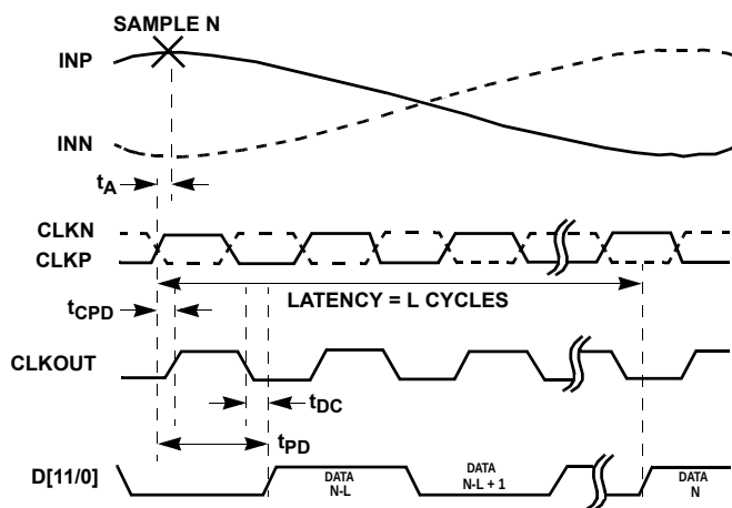
FIGURE 3B. SDR
