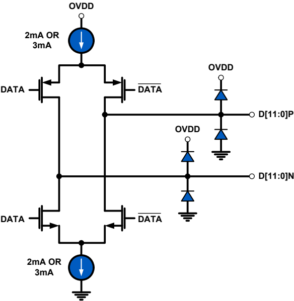
FIGURE 46. LVDS OUTPUTS
