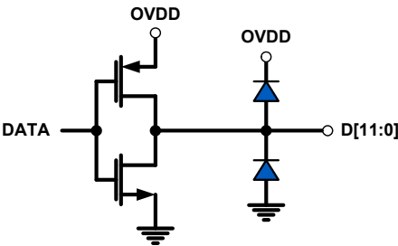
FIGURE 47. CMOS OUTPUTS
