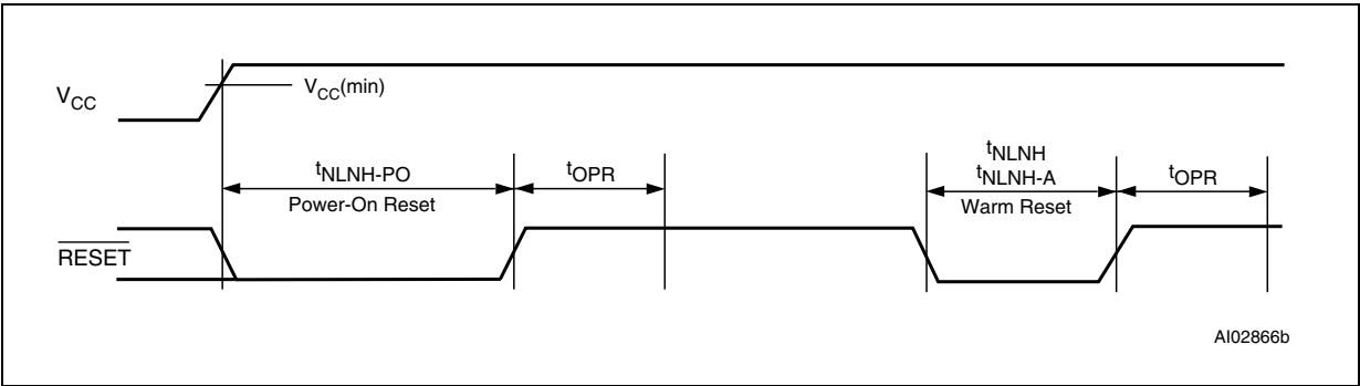
Figure 33. Reset ( \overline{\text{RESET}} ) timing
