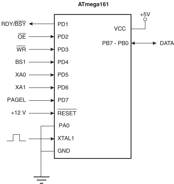
Figure 75. Parallel Programming
