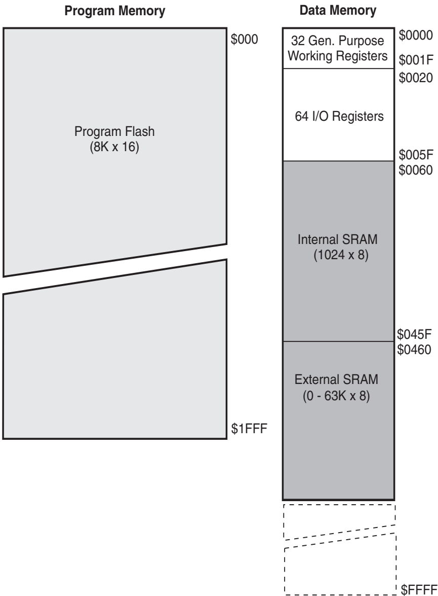
Figure 5. Memory Maps
