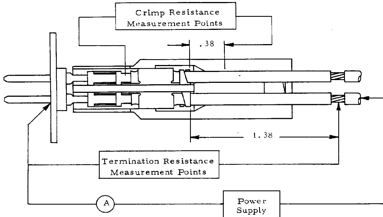
Figure 3 Resistance and Temperature Measurement Points
