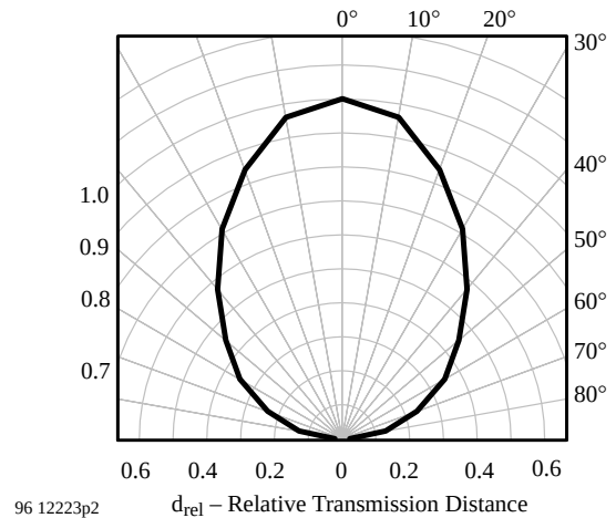
Figure 11. Directivity
