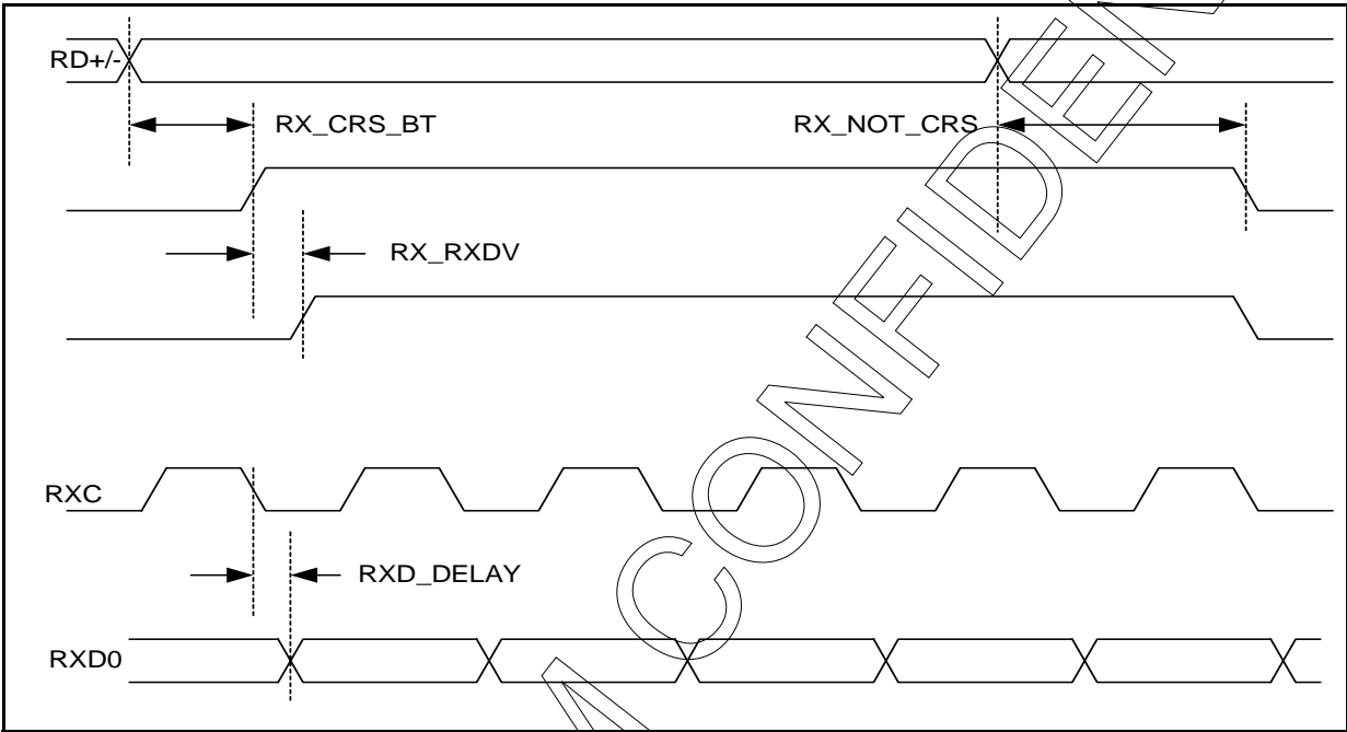
Figure 14: 10BASE-T Serial Receive Timing
