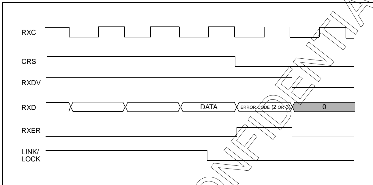
Figure 10: MII Link Failure or Stream Cipher Error During Receive Packet
