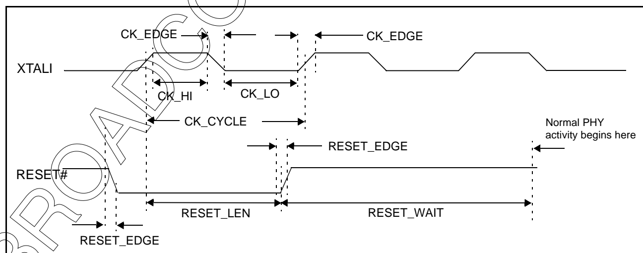
Figure 4: Clock and Reset Timing
