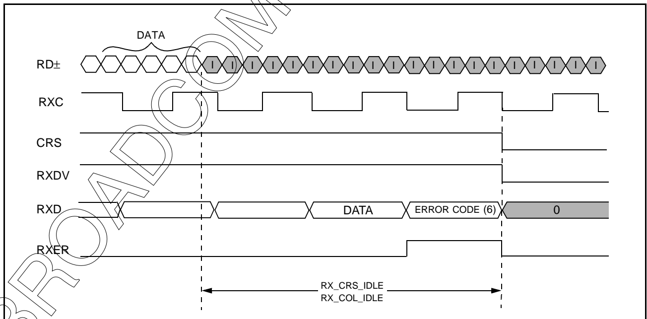
Figure 9: MII Receive Packet Premature End (100BASE-TX)
