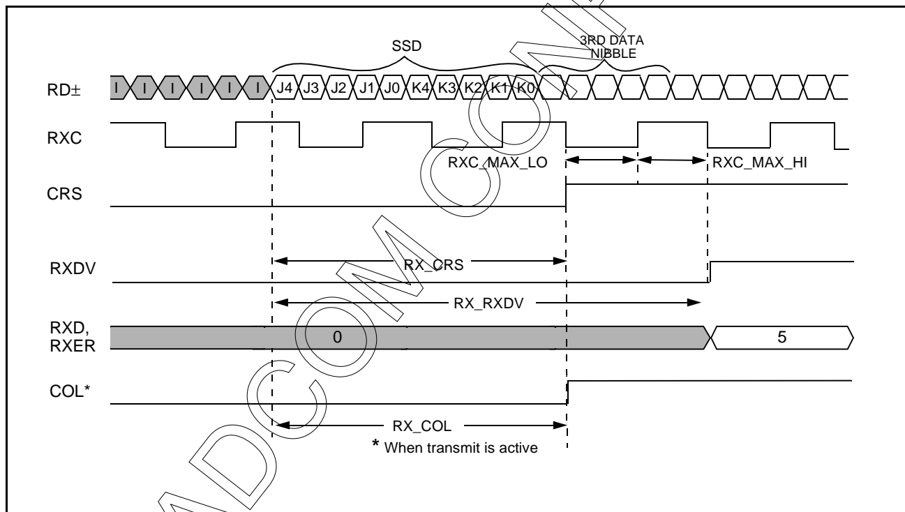
Figure 7: MII Receive Start of Packet Timing (100BASE-TX)
