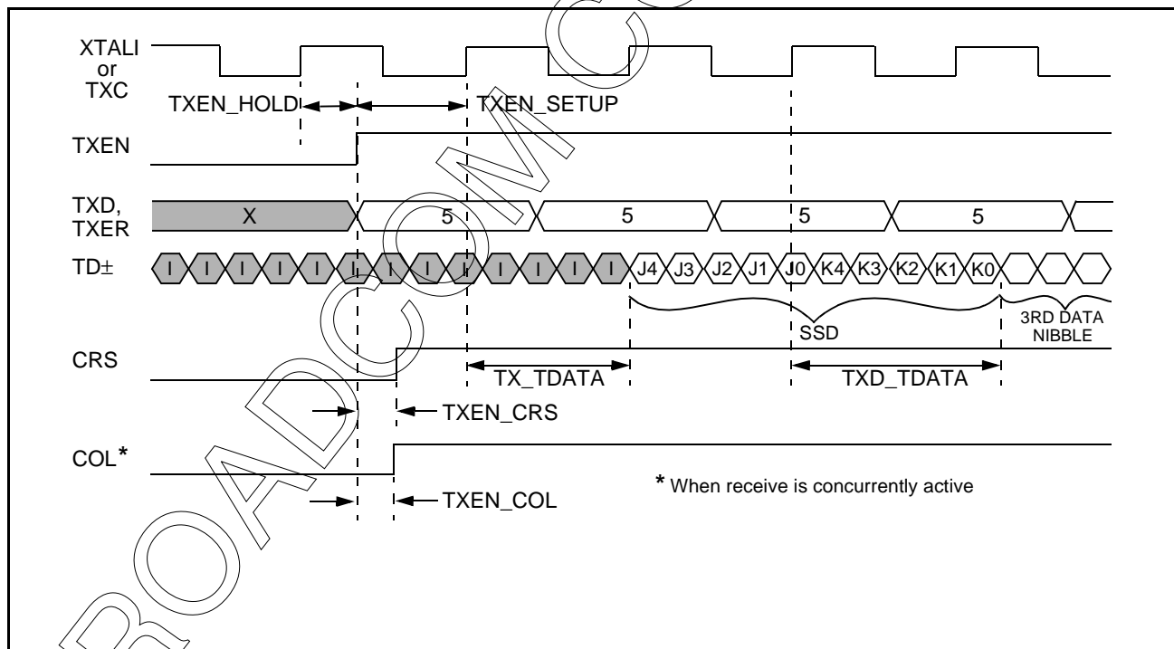
Figure 5: MII Transmit Start of Packet Timing (100BASE-TX)
