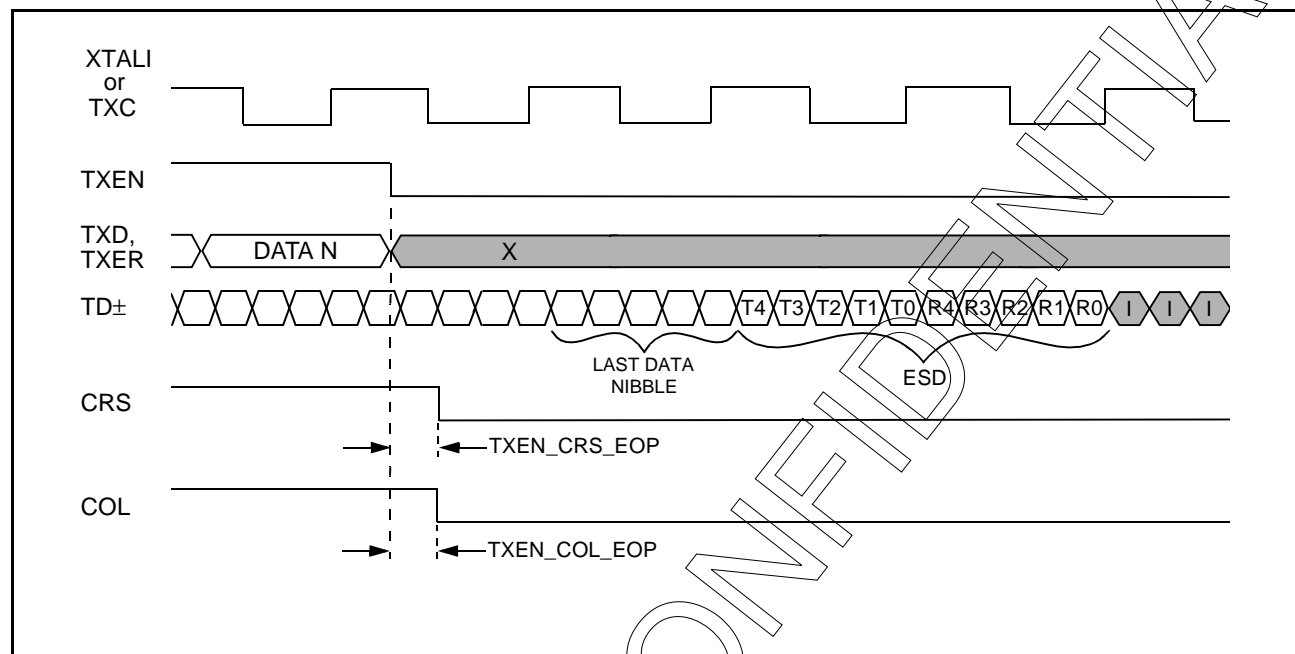
Figure 6: MII Transmit End of Packet Timing (100BASE-TX)
