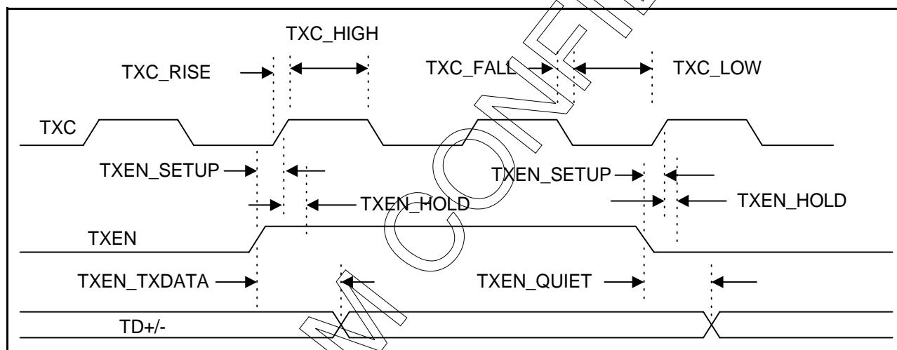
Figure 13: 10BASE-T Serial Transmit Timing
