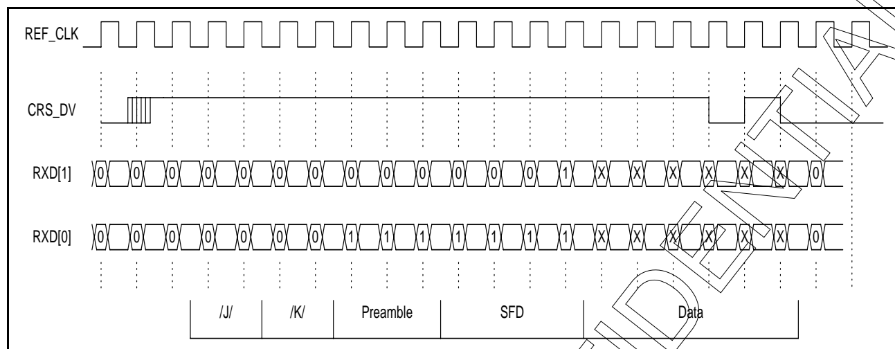
Figure 18: RMII Receive Packet Timing
