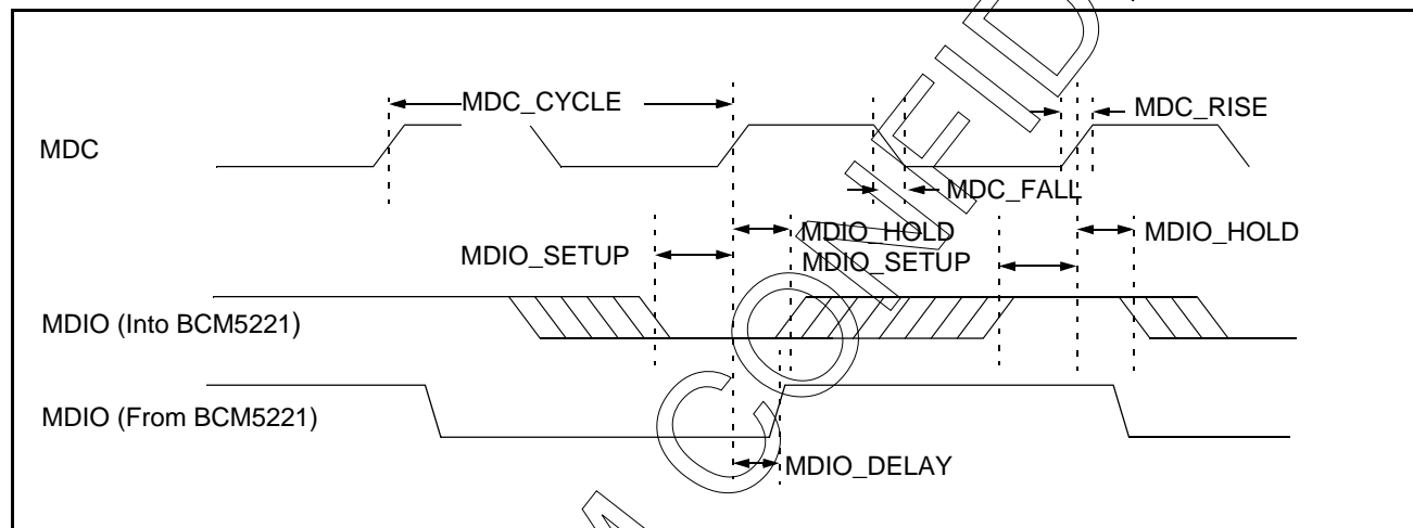
Figure 15: Management Interface Timing
