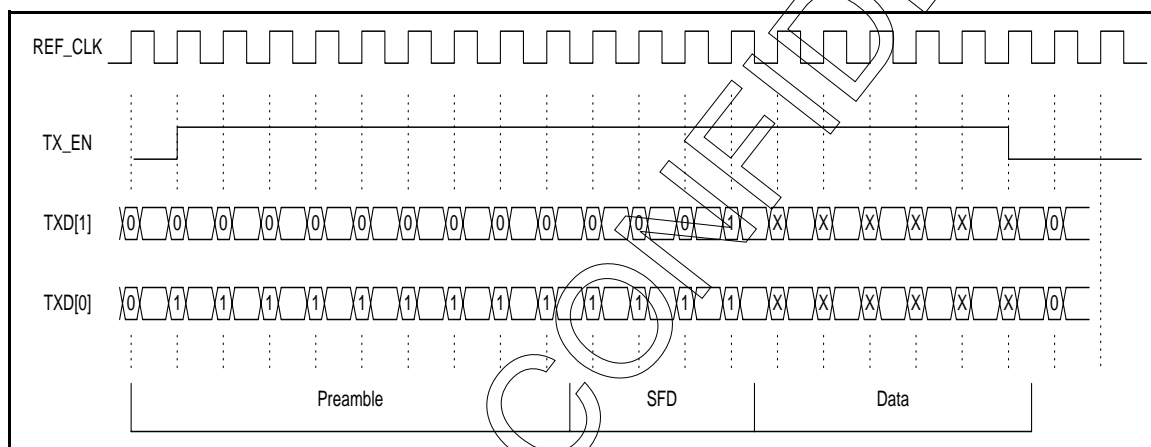
Figure 17: RMII Transmit Packet Timing
