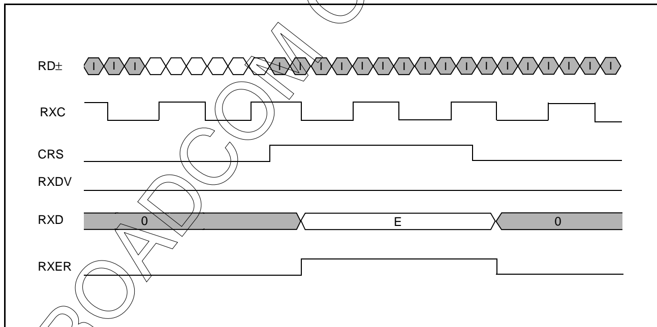
Figure 11: MII False Carrier Sense Timing (100BASE-TX)
