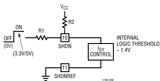
Figure 8. Partial Shutdown
