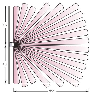
Horizontal Coverage
