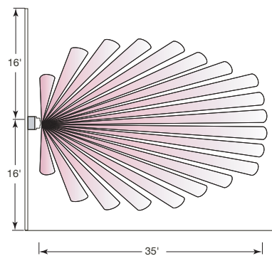
Horizontal Coverage
