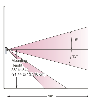
Vertical Coverage
