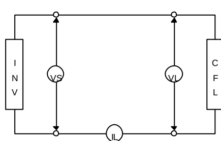
CFL Testina Circuit
