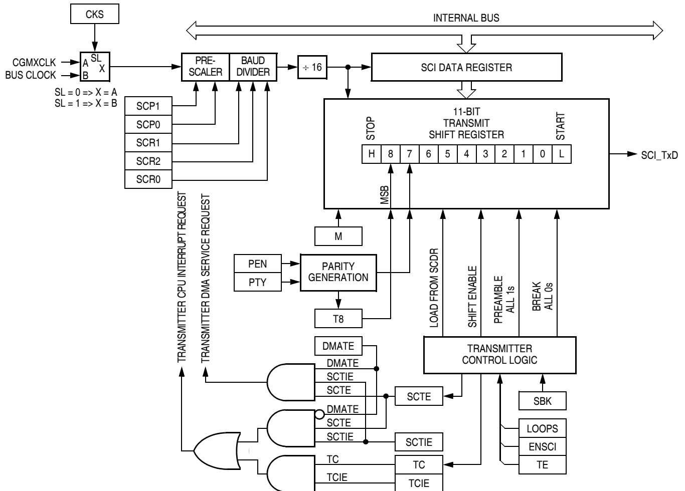
Figure 13-7. SCI Transmitter
