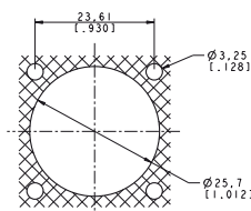
Panel Drilling
