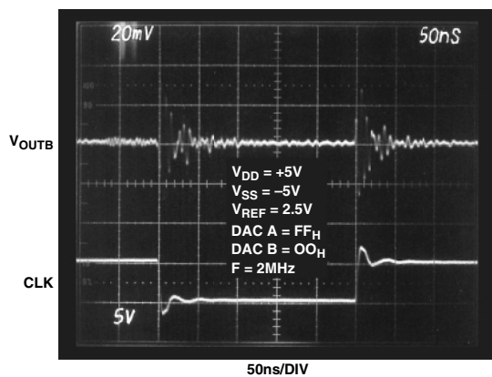
Figure 20. Digital Feedthrough
