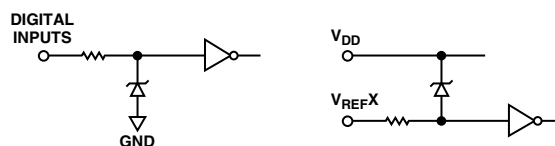
Figure 33. Equivalent ESD Protection Circuits
