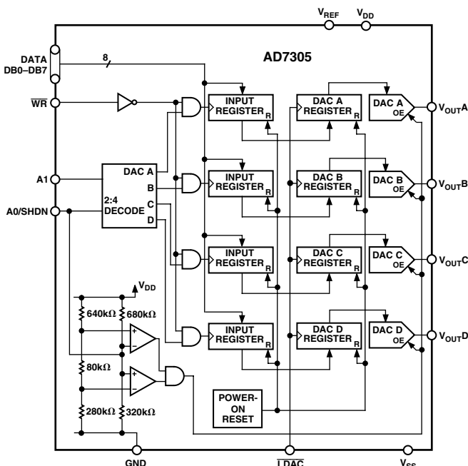
Figure 32. AD7305 Equivalent Logic Interface
