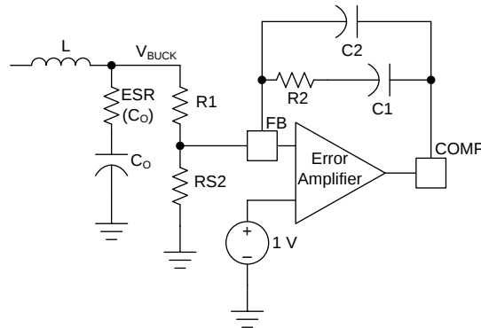
Figure 21. Type II Compensation
