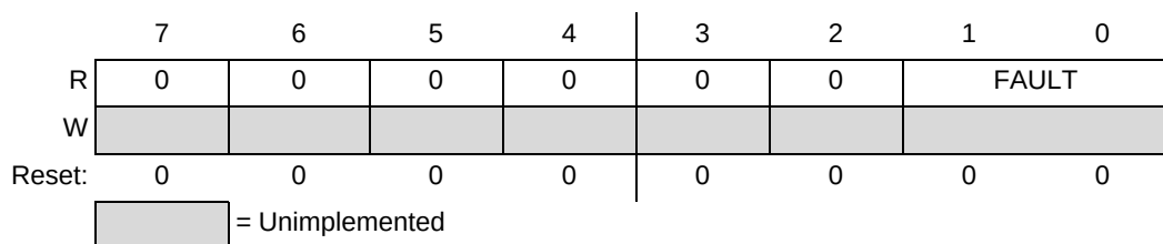
Figure 22. Fault Register
