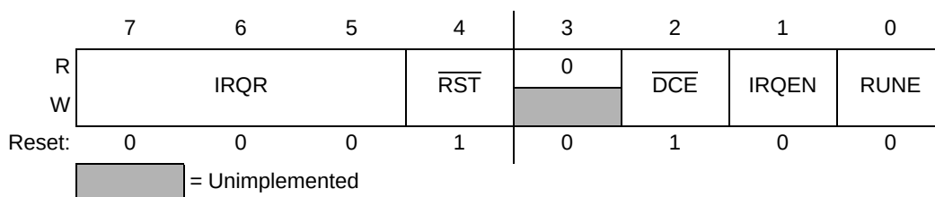
Figure 17. Configuration Register
