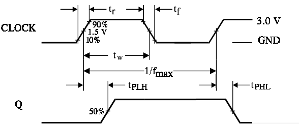
Figure 1. Switching Waveforms
