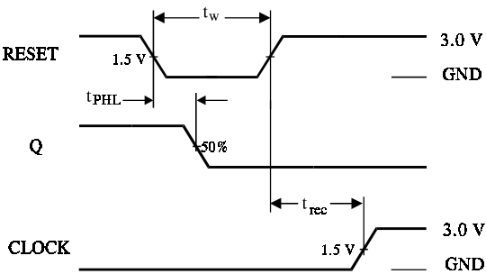
Figure 2. Switching Waveforms
