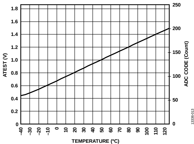
Figure 13. ATEST Voltage and ADC Code vs. Temperature
