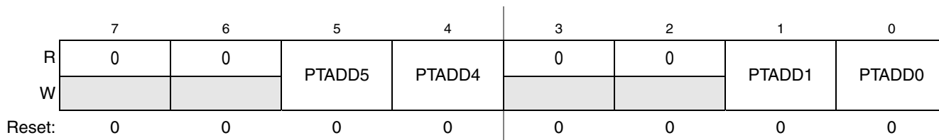
Figure 6-3. Port A Data Direction Register (PTADD)
