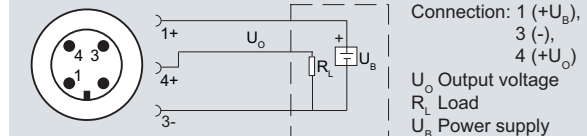
Connection with voltage output and connector M12x1
